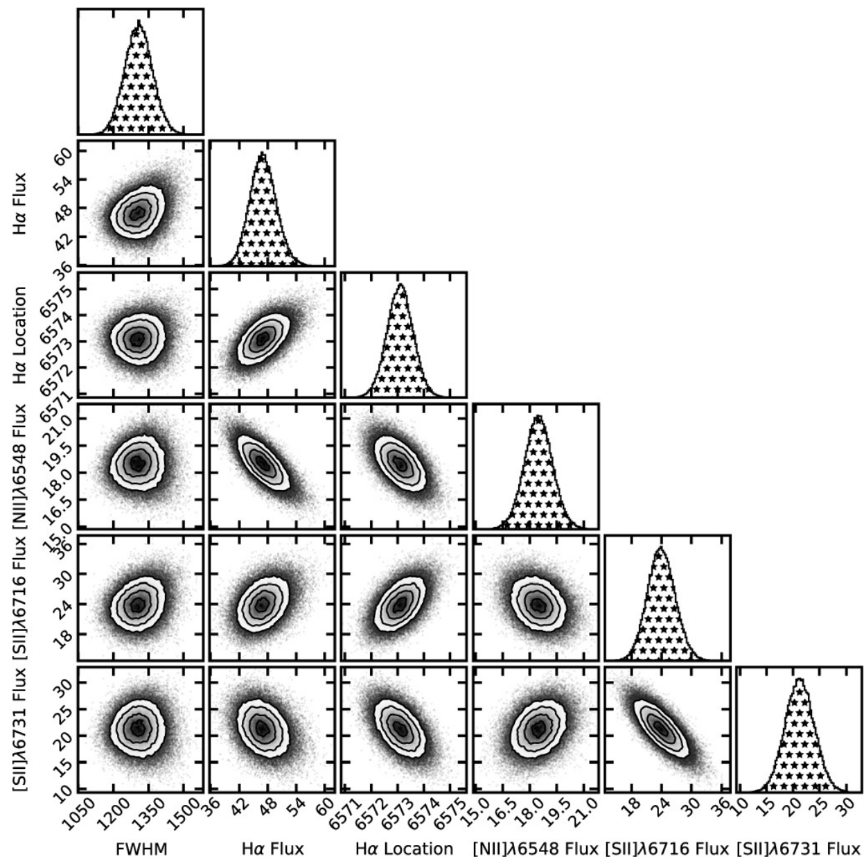
Figure 6. from Julie Hlavacek-Larrondo et al 2025 Astrophys. J. 980 doi:10.3847/1538-4357/ada7ed https://dx.doi.org/10.3847/1538-4357/ada7ed © 2025. The Author(s). Published by the American Astronomical Society.
