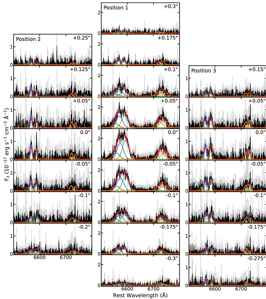
Figure 5. from Julie Hlavacek-Larrondo et al 2025 Astrophys. J. 980 doi:10.3847/1538-4357/ada7ed https://dx.doi.org/10.3847/1538-4357/ada7ed © 2025. The Author(s). Published by the American Astronomical Society.
