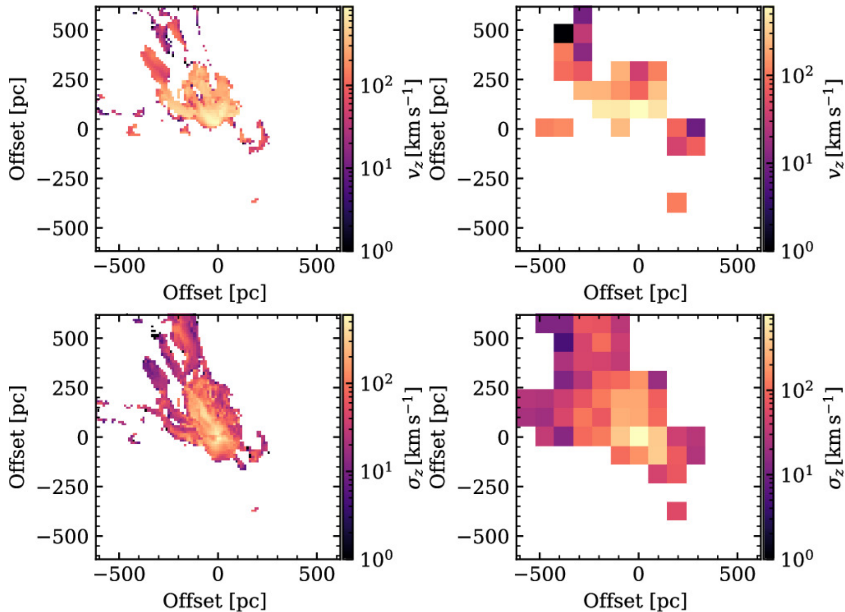
Figure 16. from Julie Hlavacek-Larrondo et al 2025 Astrophys. J. 980 doi:10.3847/1538-4357/ada7ed https://dx.doi.org/10.3847/1538-4357/ada7ed © 2025. The Author(s). Published by the American Astronomical Society.
