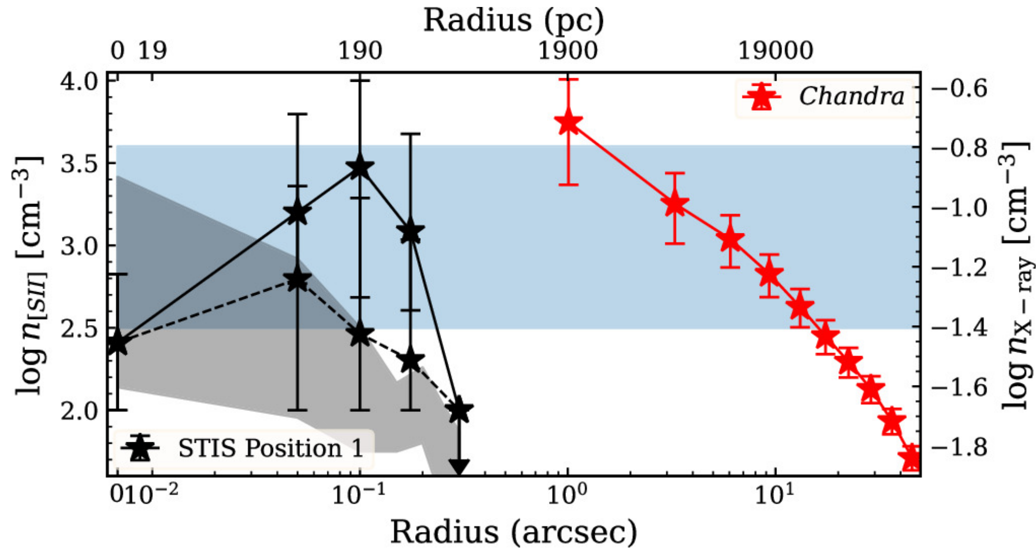
Figure 15. from Julie Hlavacek-Larrondo et al 2025 Astrophys. J. 980 doi:10.3847/1538-4357/ada7ed https://dx.doi.org/10.3847/1538-4357/ada7ed © 2025. The Author(s). Published by the American Astronomical Society.
