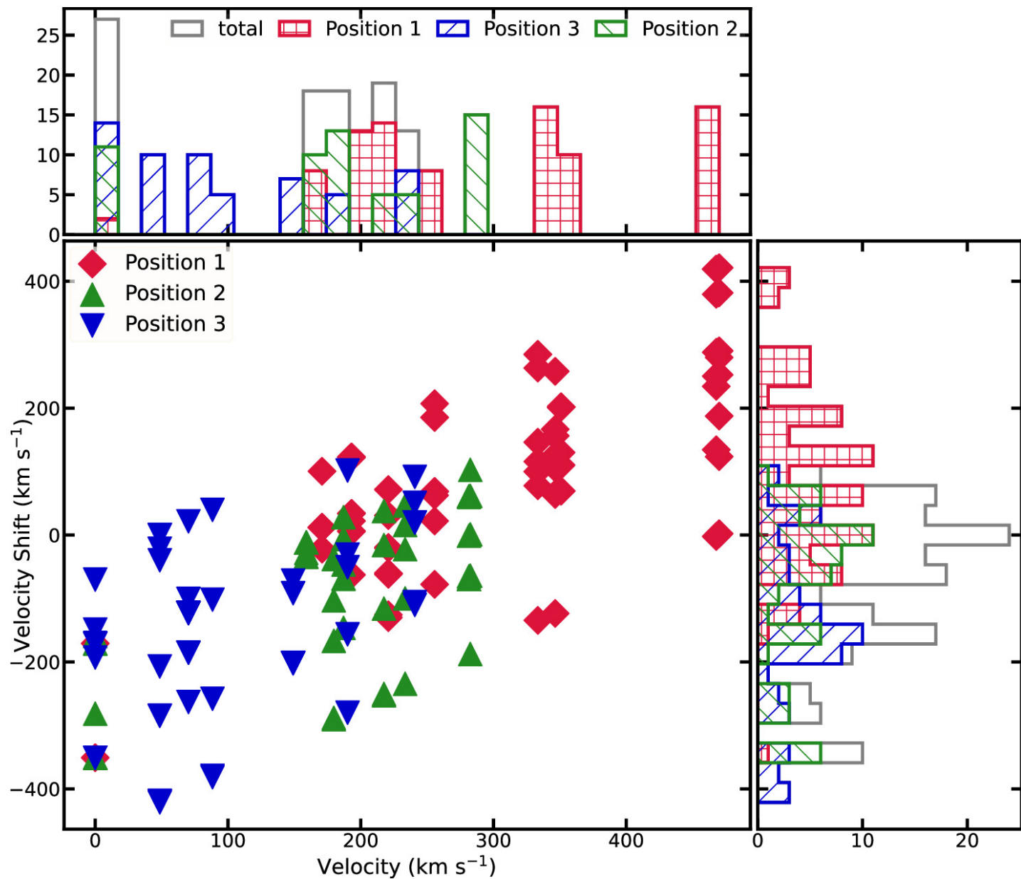
Figure 14. from Julie Hlavacek-Larrondo et al 2025 Astrophys. J. 980 doi:10.3847/1538-4357/ada7ed https://dx.doi.org/10.3847/1538-4357/ada7ed © 2025. The Author(s). Published by the American Astronomical Society.
