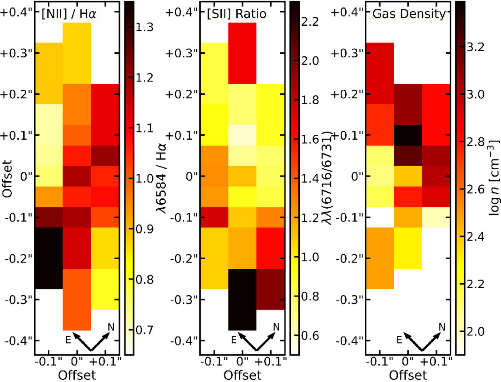
Figure 13. from Julie Hlavacek-Larrondo et al 2025 Astrophys. J. 980 doi:10.3847/1538-4357/ada7ed https://dx.doi.org/10.3847/1538-4357/ada7ed © 2025. The Author(s). Published by the American Astronomical Society.
