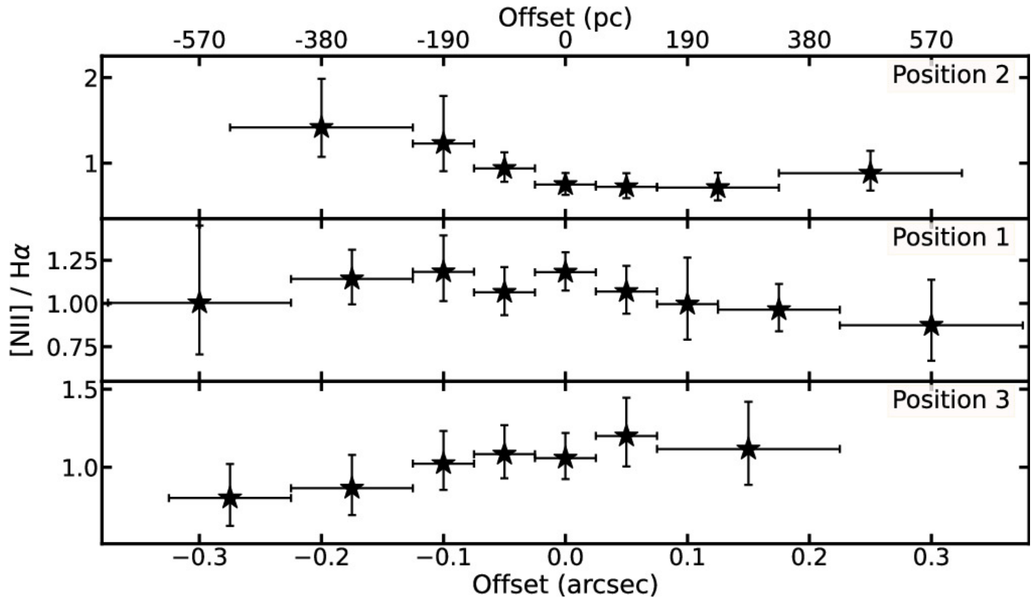
Figure 11. from Julie Hlavacek-Larrondo et al 2025 Astrophys. J. 980 doi:10.3847/1538-4357/ada7ed https://dx.doi.org/10.3847/1538-4357/ada7ed © 2025. The Author(s). Published by the American Astronomical Society.
