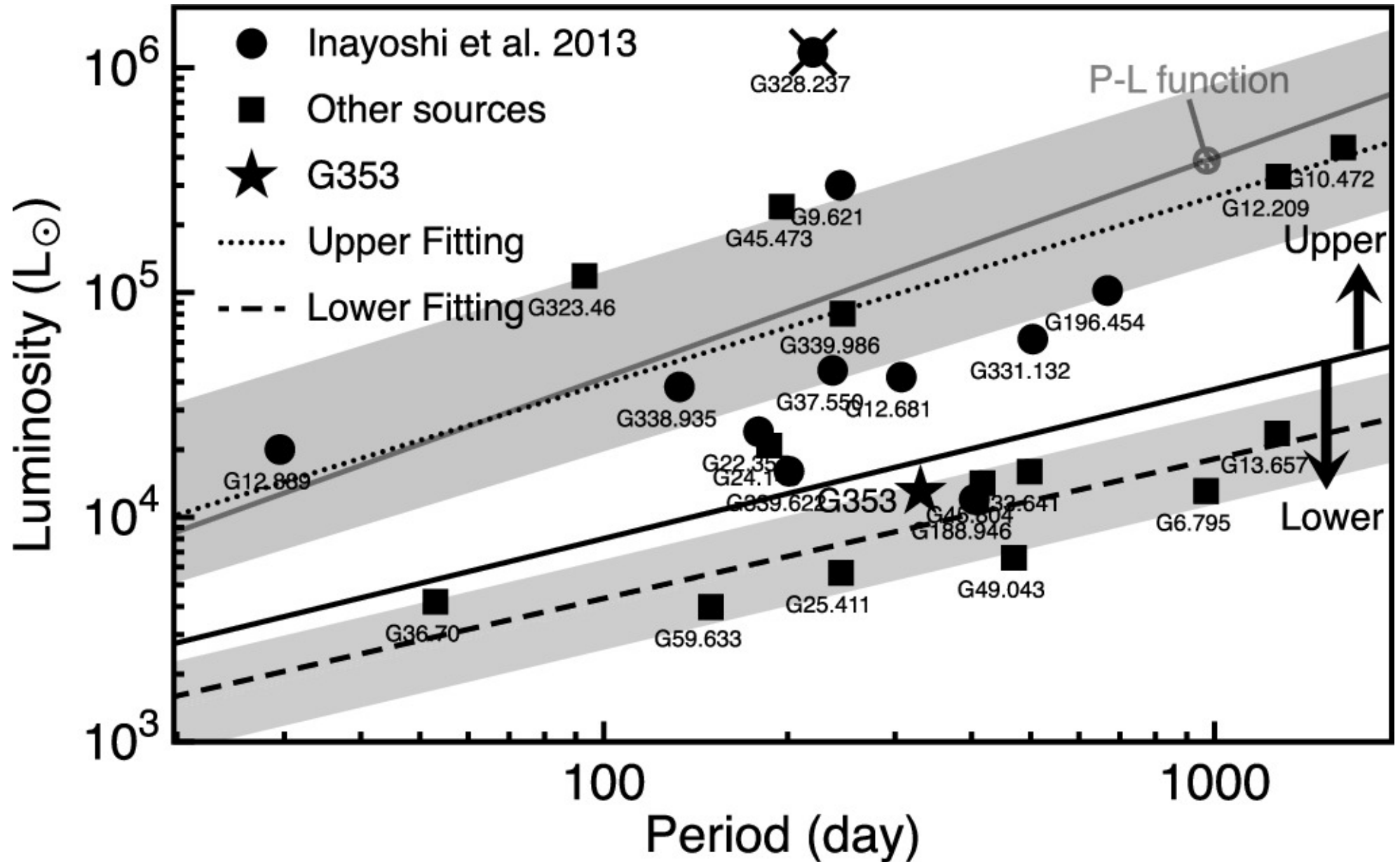
Figure 5. from Shi-Min Song et al 2025 Astrophys. J. 980 doi:10.3847/1538-4357/ada4a8 https://dx.doi.org/10.3847/1538-4357/ada4a8 © 2025. The Author(s). Published by the American Astronomical Society.
