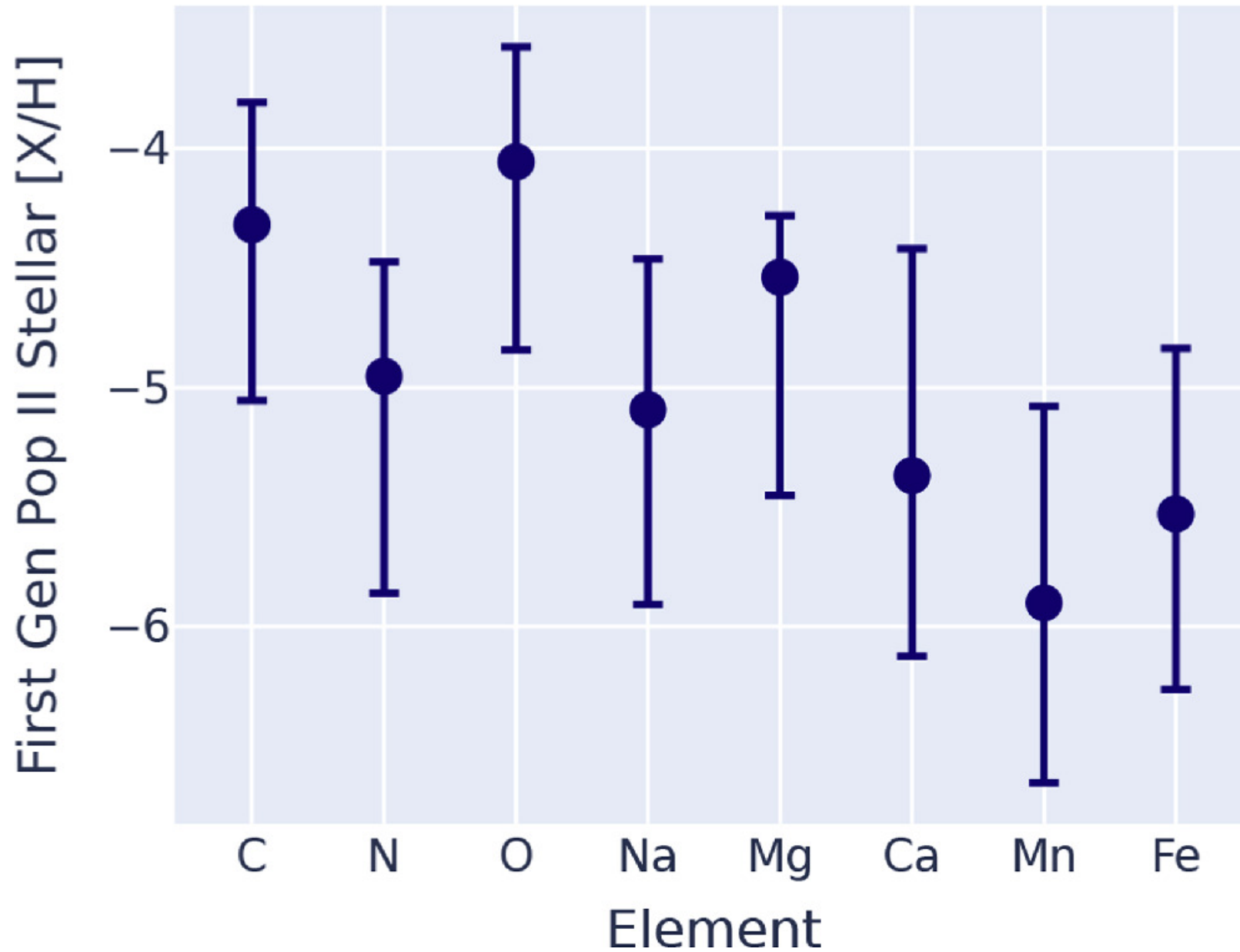
Figure 9. from Kaley Brauer et al 2025 Astrophys. J. 980 doi:10.3847/1538-4357/ada4a1 https://dx.doi.org/10.3847/1538-4357/ada4a1 © 2025. The Author(s). Published by the American Astronomical Society.
