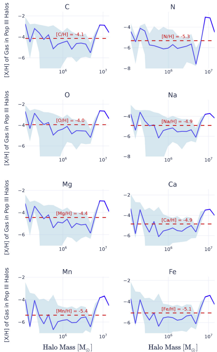
Figure 8. from Kaley Brauer et al 2025 Astrophys. J. 980 doi:10.3847/1538-4357/ada4a1 https://dx.doi.org/10.3847/1538-4357/ada4a1 © 2025. The Author(s). Published by the American Astronomical Society.
