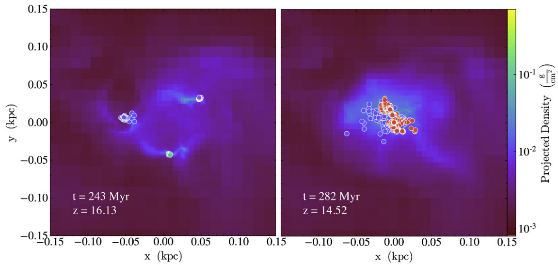
Figure 5. from Kaley Brauer et al 2025 Astrophys. J. 980 doi:10.3847/1538-4357/ada4a1 https://dx.doi.org/10.3847/1538-4357/ada4a1 © 2025. The Author(s). Published by the American Astronomical Society.
