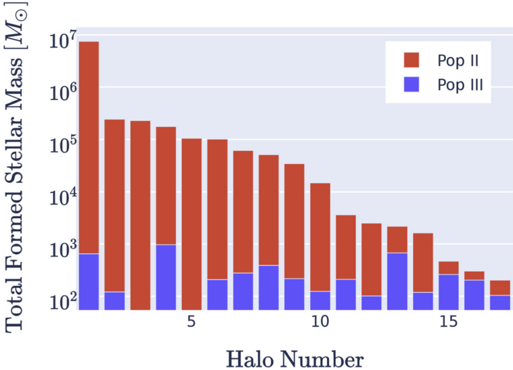
Figure 3. from Kaley Brauer et al 2025 Astrophys. J. 980 doi:10.3847/1538-4357/ada4a1 https://dx.doi.org/10.3847/1538-4357/ada4a1 © 2025. The Author(s). Published by the American Astronomical Society.
