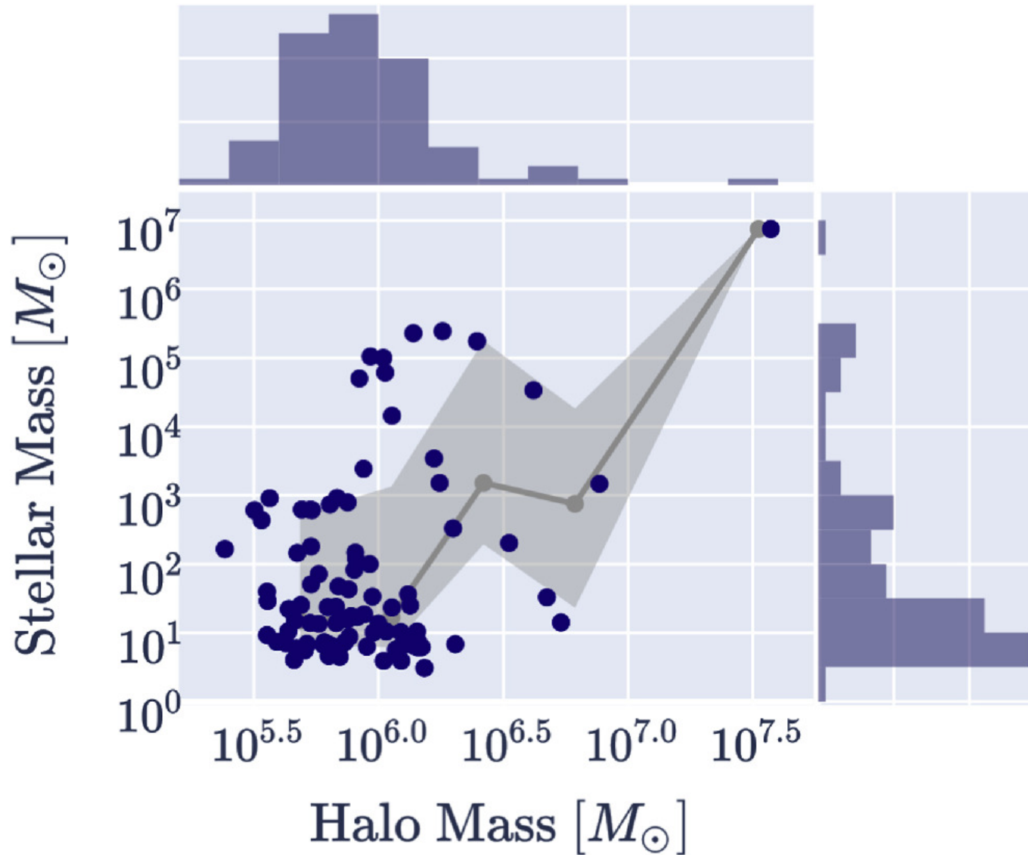
Figure 2. from Kaley Brauer et al 2025 Astrophys. J. 980 doi:10.3847/1538-4357/ada4a1 https://dx.doi.org/10.3847/1538-4357/ada4a1 © 2025. The Author(s). Published by the American Astronomical Society.
