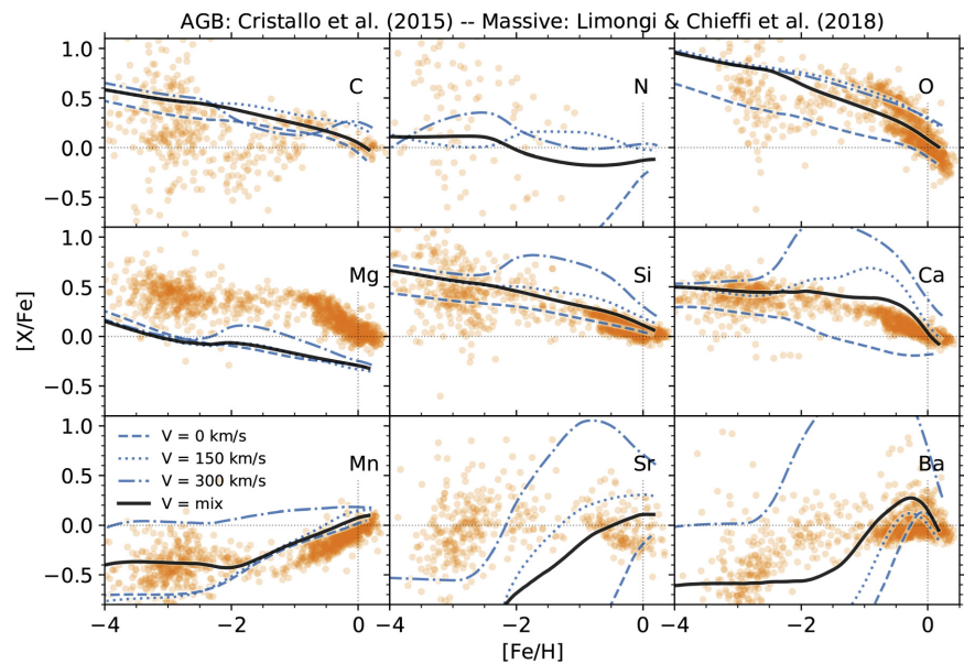
Figure A3. from Kaley Brauer et al 2025 Astrophys. J. 980 doi:10.3847/1538-4357/ada4a1 https://dx.doi.org/10.3847/1538-4357/ada4a1 © 2025. The Author(s). Published by the American Astronomical Society.
