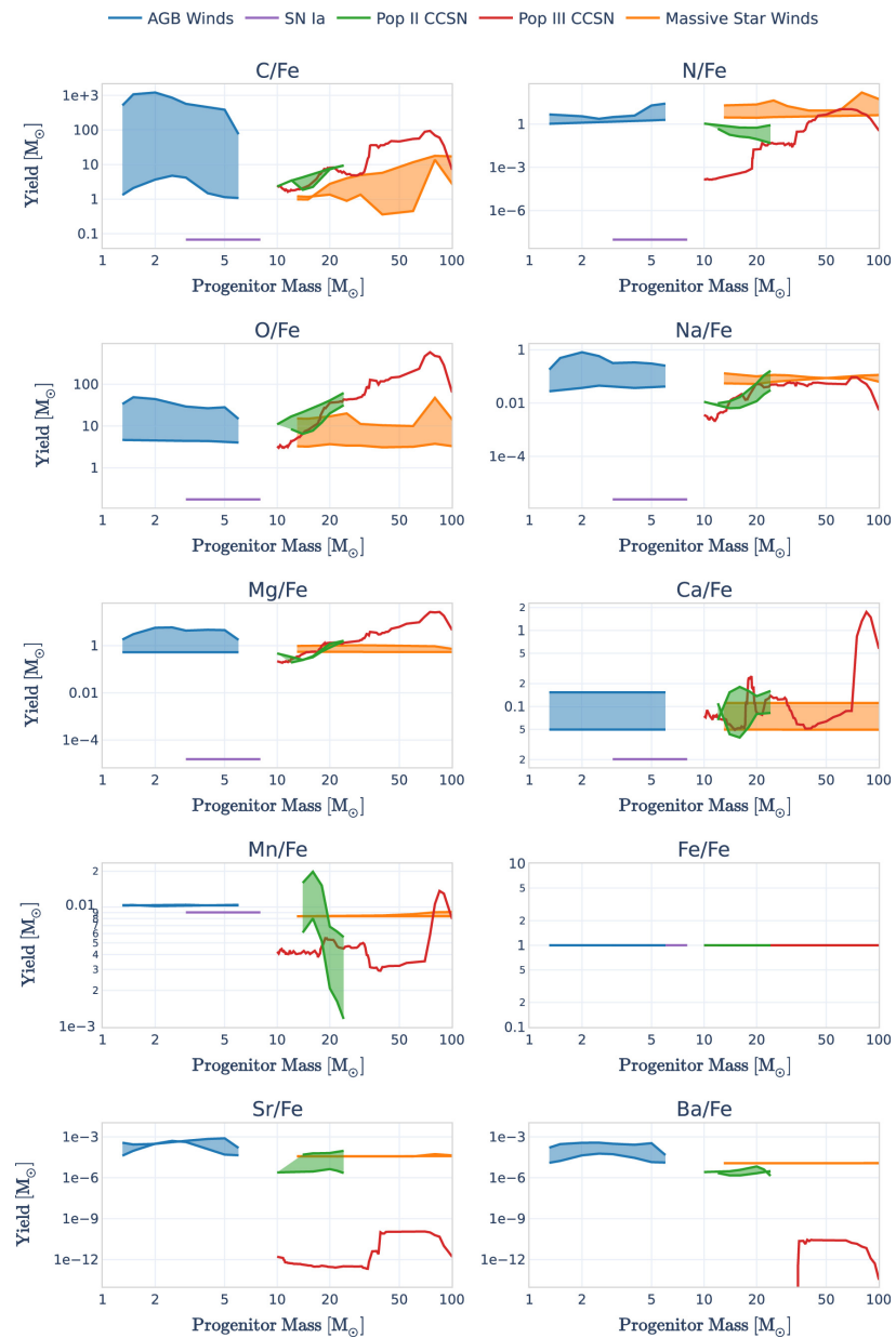
Figure A2. from Kaley Brauer et al 2025 Astrophys. J. 980 doi:10.3847/1538-4357/ada4a1 https://dx.doi.org/10.3847/1538-4357/ada4a1 © 2025. The Author(s). Published by the American Astronomical Society.
