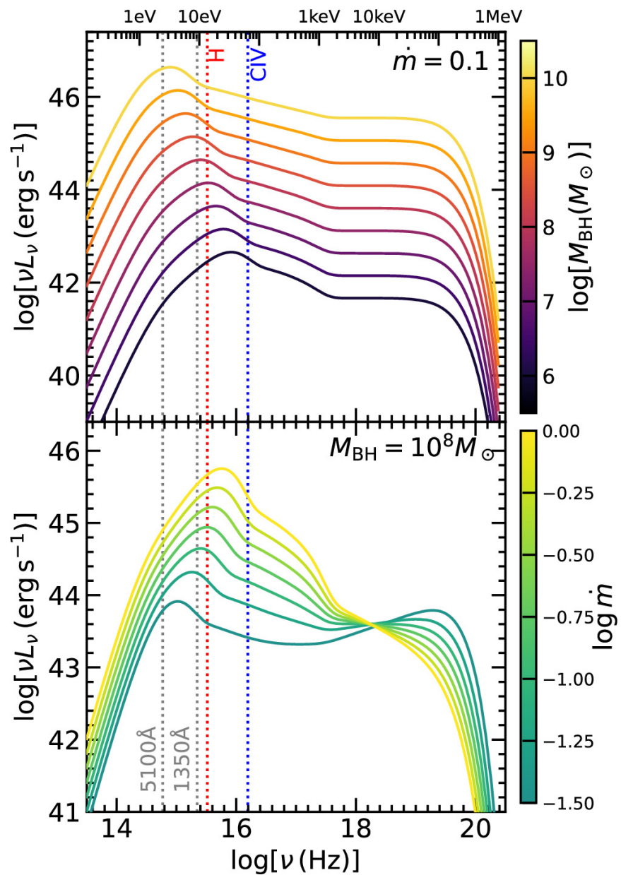
Figure 1. from Qiaoya Wu et al 2025 Astrophys. J. 980 doi:10.3847/1538-4357/ada386 https://dx.doi.org/10.3847/1538-4357/ada386 © 2025. The Author(s). Published by the American Astronomical Society.
