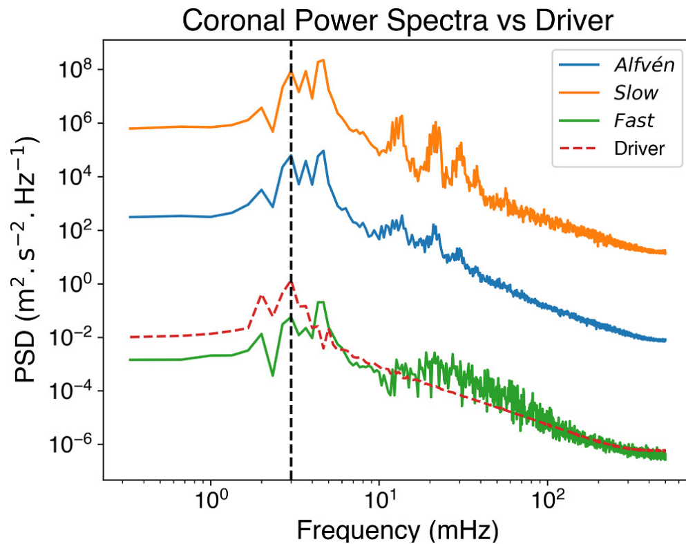
Figure 8. from Hemanthi Miriyala et al 2025 Astrophys. J. 979 doi:10.3847/1538-4357/ada26f https://dx.doi.org/10.3847/1538-4357/ada26f © 2025. The Author(s). Published by the American Astronomical Society.
