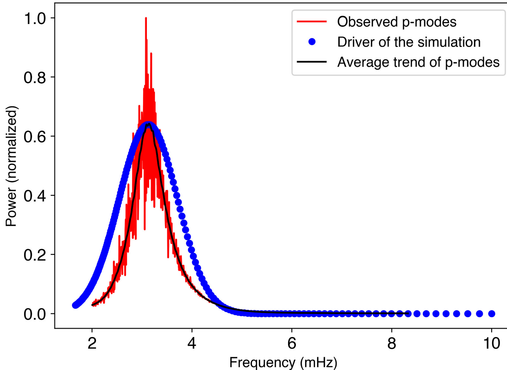
Figure 4. from Hemanthi Miriyala et al 2025 Astrophys. J. 979 doi:10.3847/1538-4357/ada26f https://dx.doi.org/10.3847/1538-4357/ada26f © 2025. The Author(s). Published by the American Astronomical Society.
