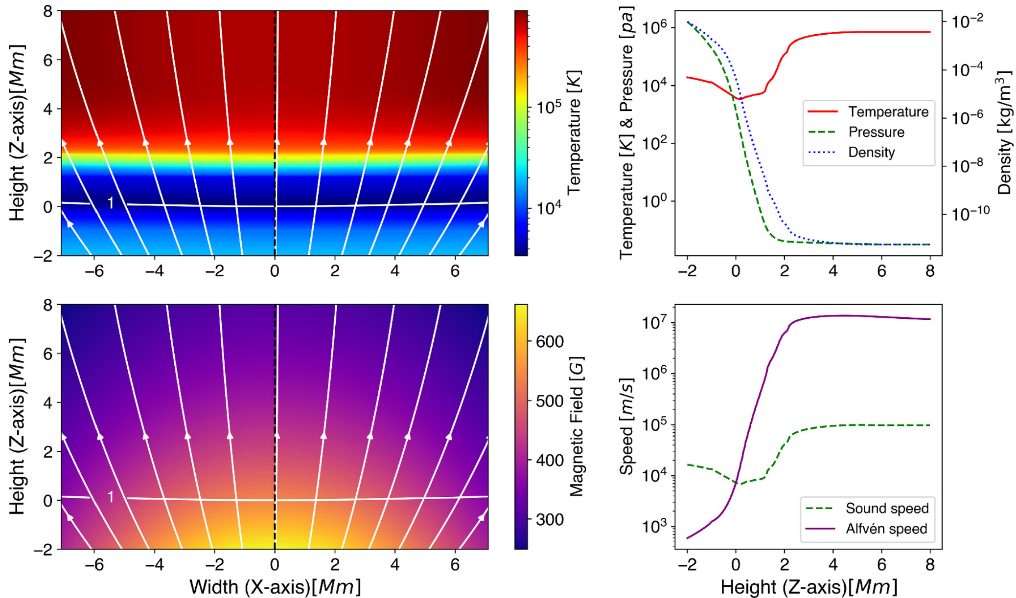
Figure 2. from Hemanthi Miriyala et al 2025 Astrophys. J. 979 doi:10.3847/1538-4357/ada26f https://dx.doi.org/10.3847/1538-4357/ada26f © 2025. The Author(s). Published by the American Astronomical Society.
