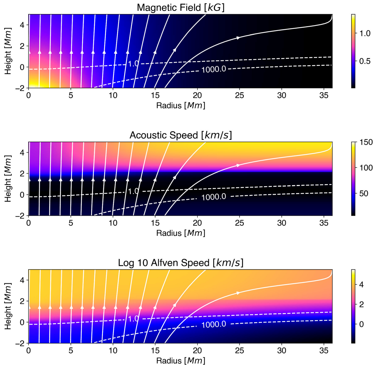
Figure 1. from Hemanthi Miriyala et al 2025 Astrophys. J. 979 doi:10.3847/1538-4357/ada26f https://dx.doi.org/10.3847/1538-4357/ada26f © 2025. The Author(s). Published by the American Astronomical Society.
