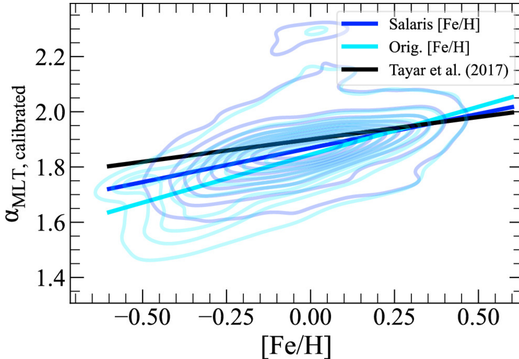
Figure 8. from Amanda L. Ash et al 2025 Astrophys. J. 979 doi:10.3847/1538-4357/ad9b18 https://dx.doi.org/10.3847/1538-4357/ad9b18 © 2025. The Author(s). Published by the American Astronomical Society.
