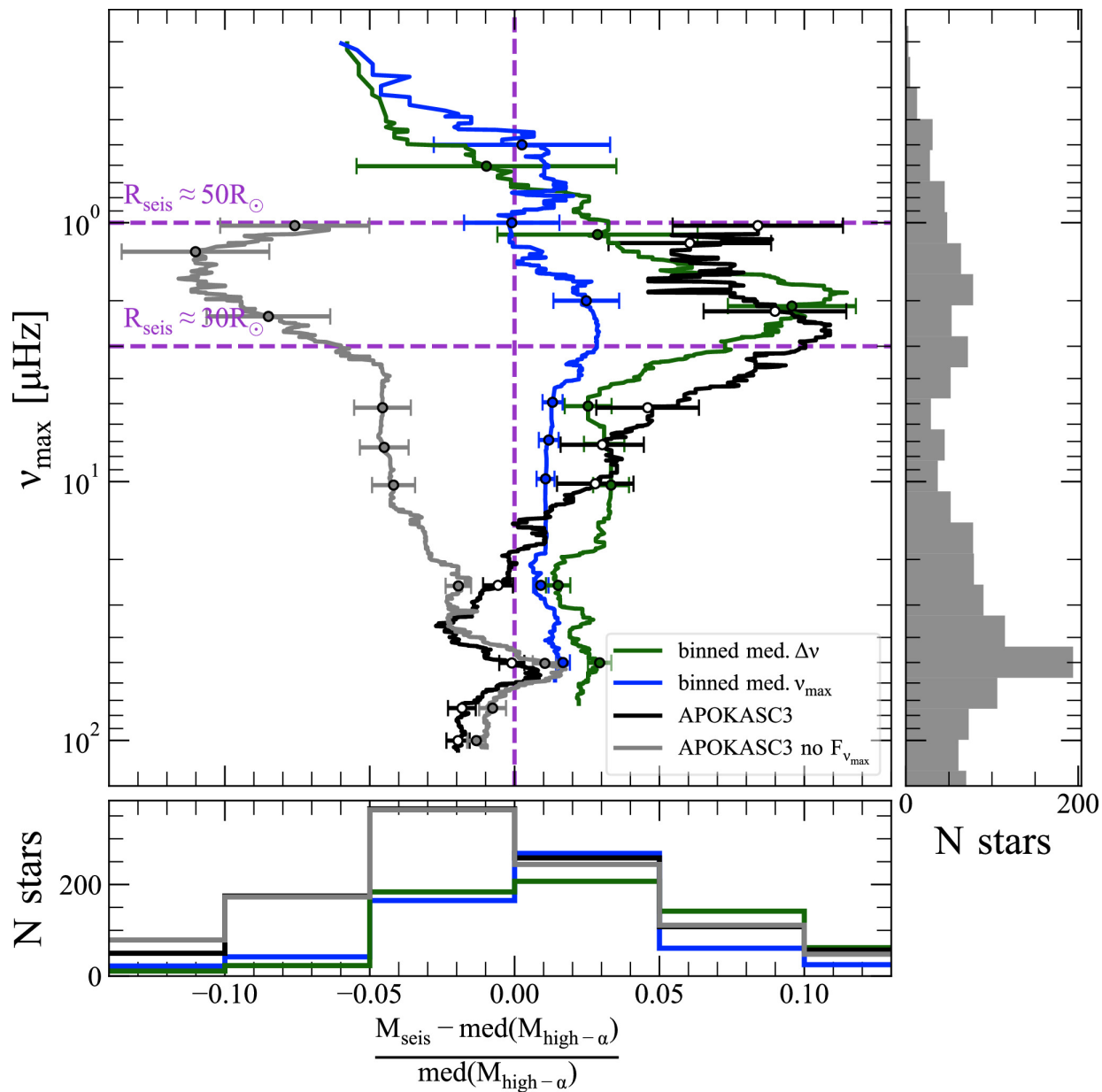
Figure 5. from Amanda L. Ash et al 2025 Astrophys. J. 979 doi:10.3847/1538-4357/ad9b18 https://dx.doi.org/10.3847/1538-4357/ad9b18 © 2025. The Author(s). Published by the American Astronomical Society.
