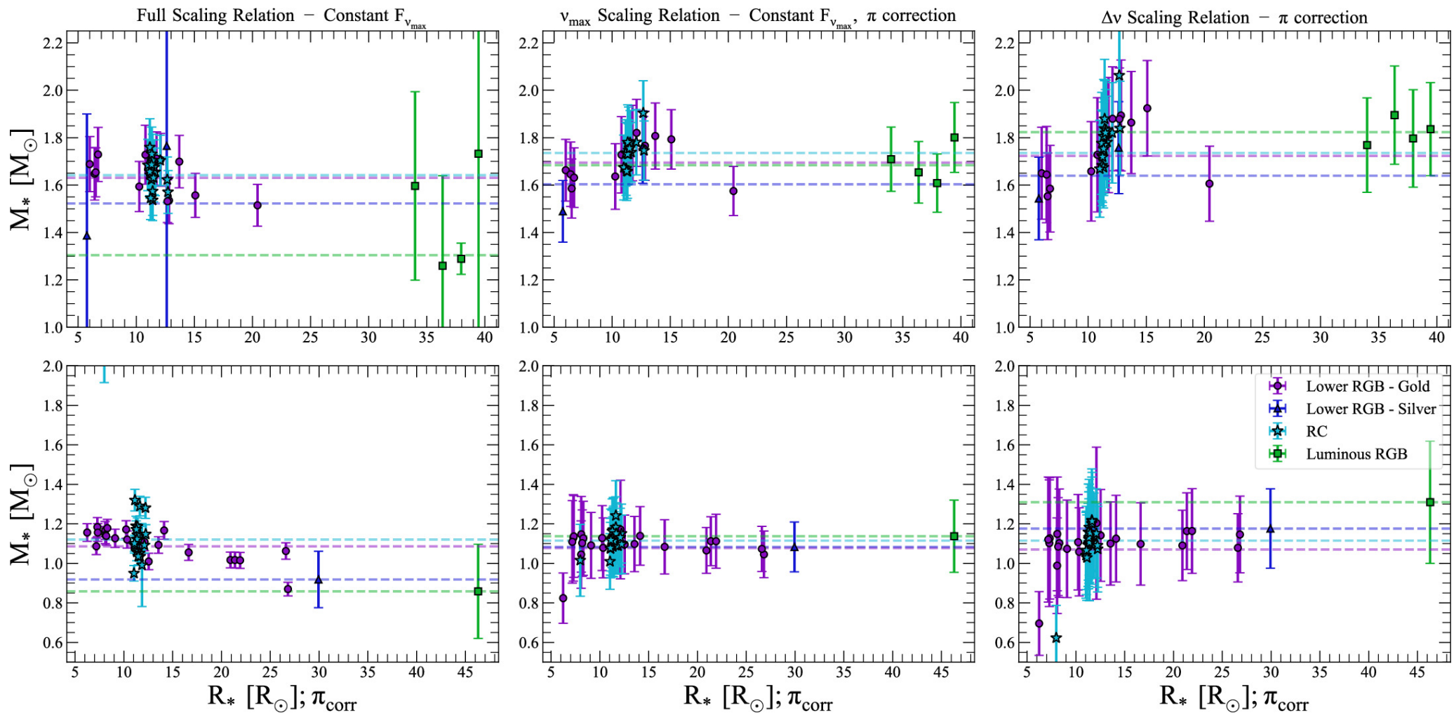
Figure 4. from Amanda L. Ash et al 2025 Astrophys. J. 979 doi:10.3847/1538-4357/ad9b18 https://dx.doi.org/10.3847/1538-4357/ad9b18 © 2025. The Author(s). Published by the American Astronomical Society.
