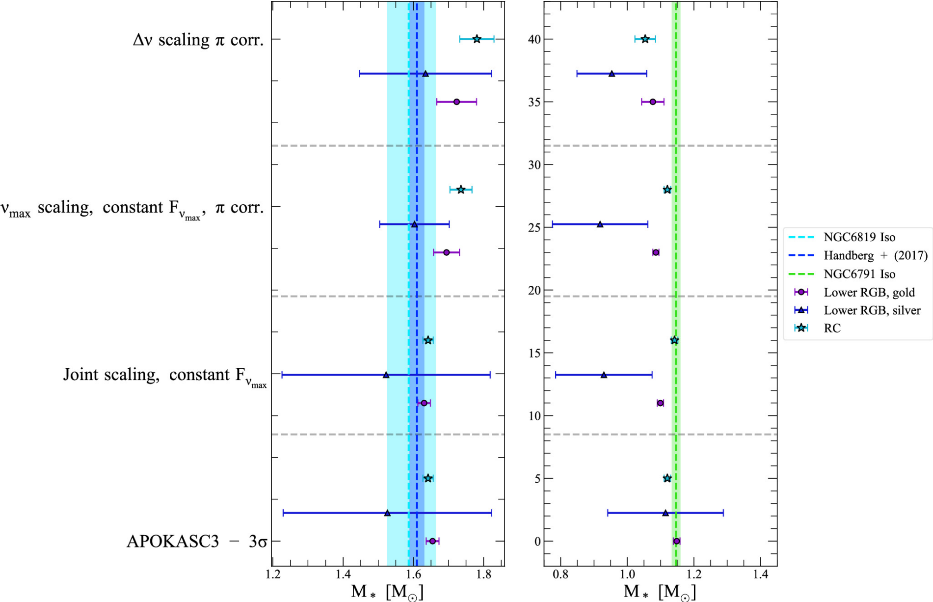
Figure 3. from Amanda L. Ash et al 2025 Astrophys. J. 979 doi:10.3847/1538-4357/ad9b18 https://dx.doi.org/10.3847/1538-4357/ad9b18 © 2025. The Author(s). Published by the American Astronomical Society.
