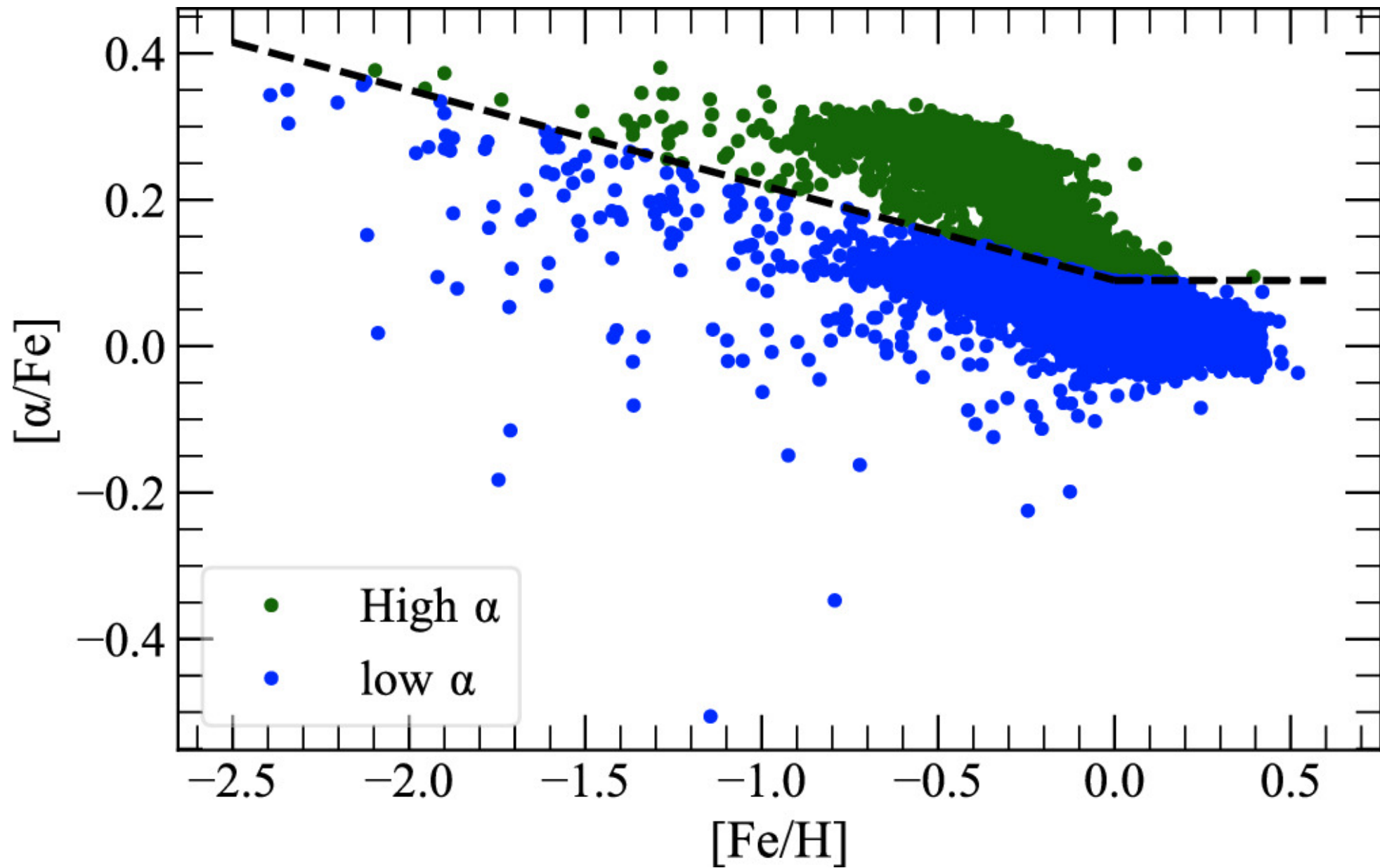
Figure 2. from Amanda L. Ash et al 2025 Astrophys. J. 979 doi:10.3847/1538-4357/ad9b18 https://dx.doi.org/10.3847/1538-4357/ad9b18 © 2025. The Author(s). Published by the American Astronomical Society.
