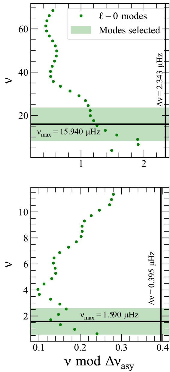
Figure 15. from Amanda L. Ash et al 2025 Astrophys. J. 979 doi:10.3847/1538-4357/ad9b18 https://dx.doi.org/10.3847/1538-4357/ad9b18 © 2025. The Author(s). Published by the American Astronomical Society.
