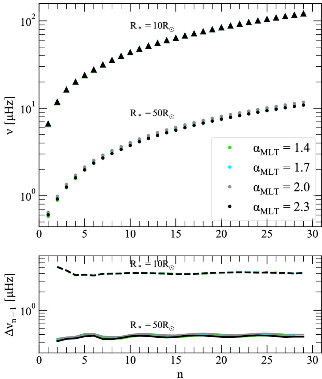
Figure 14. from Amanda L. Ash et al 2025 Astrophys. J. 979 doi:10.3847/1538-4357/ad9b18 https://dx.doi.org/10.3847/1538-4357/ad9b18 © 2025. The Author(s). Published by the American Astronomical Society.
