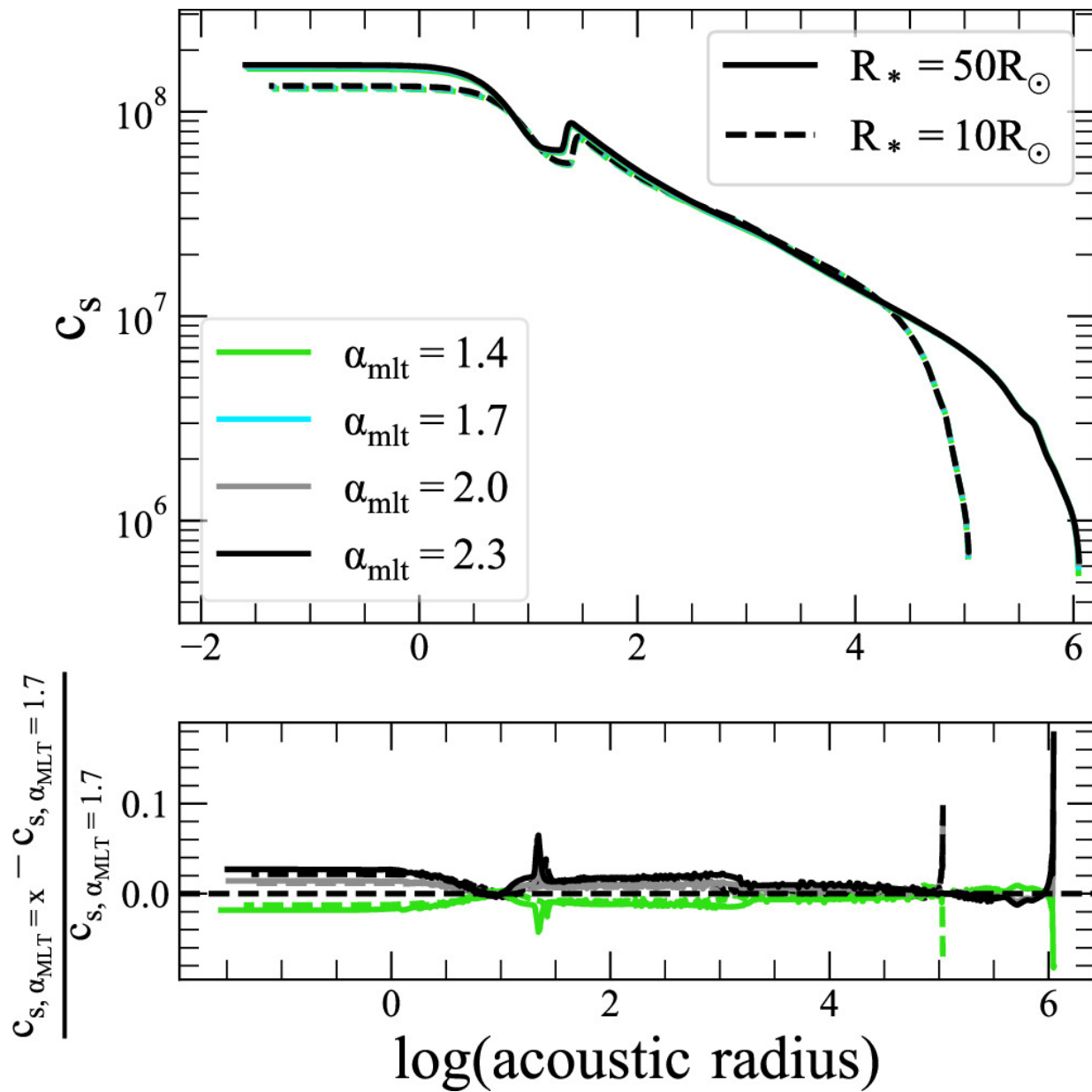
Figure 13. from Amanda L. Ash et al 2025 Astrophys. J. 979 doi:10.3847/1538-4357/ad9b18 https://dx.doi.org/10.3847/1538-4357/ad9b18 © 2025. The Author(s). Published by the American Astronomical Society.
