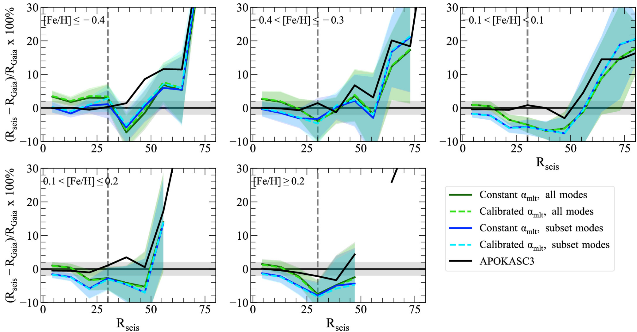
Figure 12. from Amanda L. Ash et al 2025 Astrophys. J. 979 doi:10.3847/1538-4357/ad9b18 https://dx.doi.org/10.3847/1538-4357/ad9b18 © 2025. The Author(s). Published by the American Astronomical Society.
