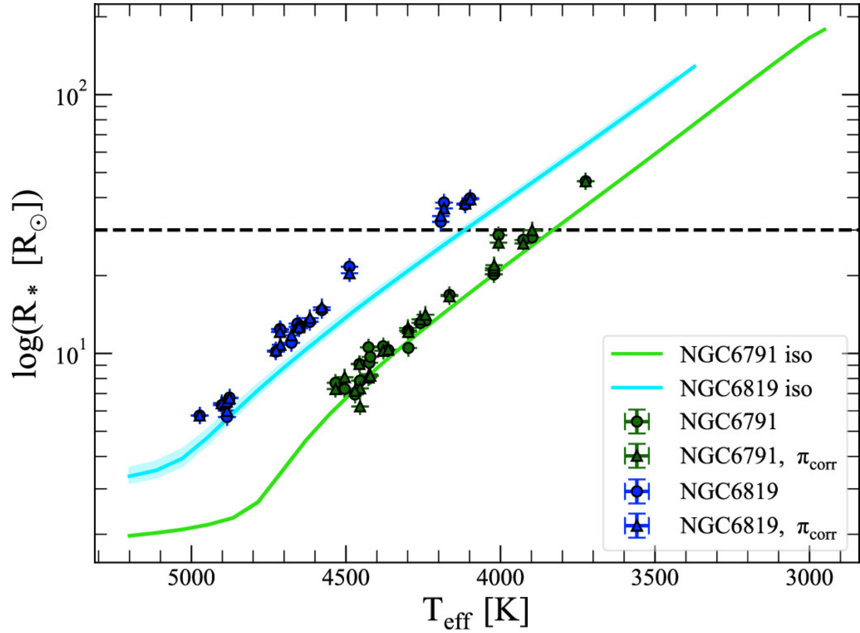
Figure 1. from Amanda L. Ash et al 2025 Astrophys. J. 979 doi:10.3847/1538-4357/ad9b18 https://dx.doi.org/10.3847/1538-4357/ad9b18 © 2025. The Author(s). Published by the American Astronomical Society.
