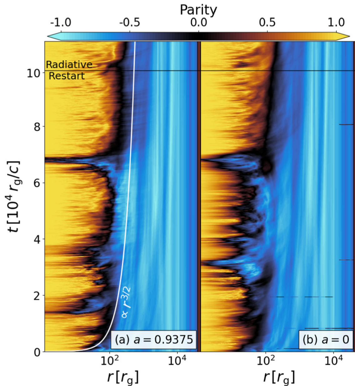
Figure 8. from Nicholas Kaaz et al 2025 Astrophys. J. 979 doi:10.3847/1538-4357/ad9a86 https://dx.doi.org/10.3847/1538-4357/ad9a86 © 2025. The Author(s). Published by the American Astronomical Society.
