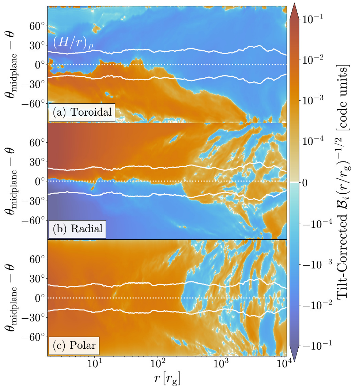
Figure 7. from Nicholas Kaaz et al 2025 Astrophys. J. 979 doi:10.3847/1538-4357/ad9a86 https://dx.doi.org/10.3847/1538-4357/ad9a86 © 2025. The Author(s). Published by the American Astronomical Society.
