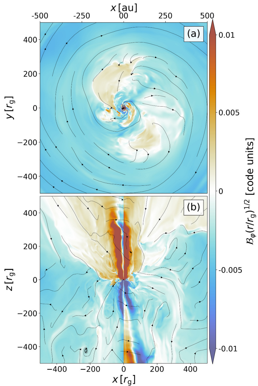
Figure 6. from Nicholas Kaaz et al 2025 Astrophys. J. 979 doi:10.3847/1538-4357/ad9a86 https://dx.doi.org/10.3847/1538-4357/ad9a86 © 2025. The Author(s). Published by the American Astronomical Society.
