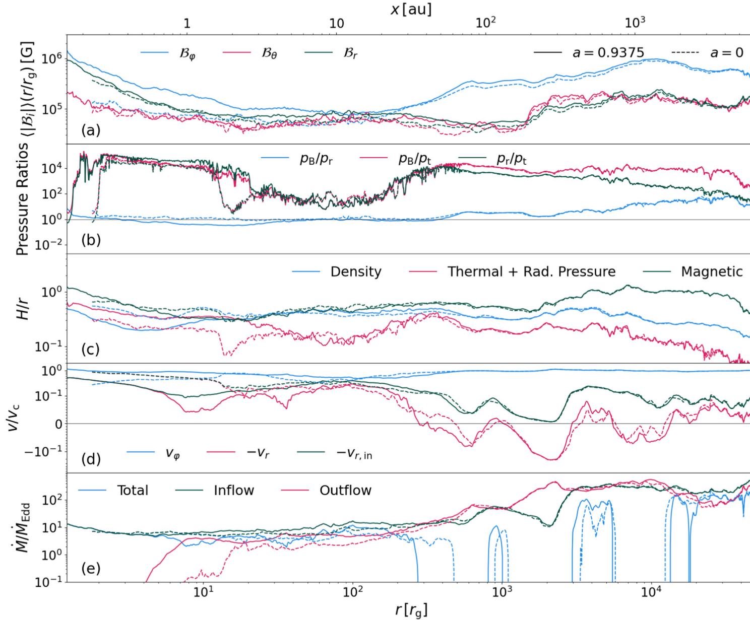
Figure 5. from Nicholas Kaaz et al 2025 Astrophys. J. 979 doi:10.3847/1538-4357/ad9a86 https://dx.doi.org/10.3847/1538-4357/ad9a86 © 2025. The Author(s). Published by the American Astronomical Society.
