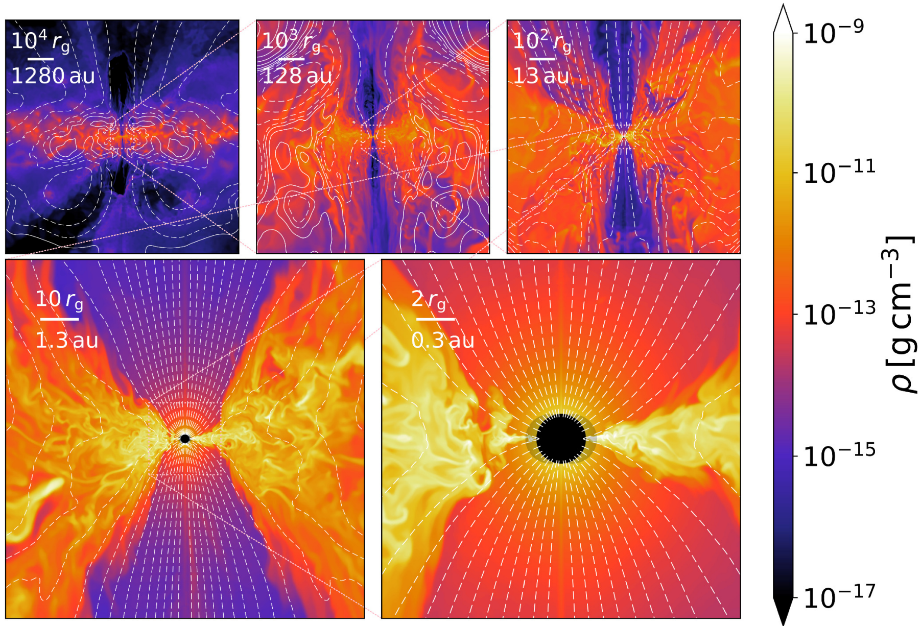
Figure 2. from Nicholas Kaaz et al 2025 Astrophys. J. 979 doi:10.3847/1538-4357/ad9a86 https://dx.doi.org/10.3847/1538-4357/ad9a86 © 2025. The Author(s). Published by the American Astronomical Society.
