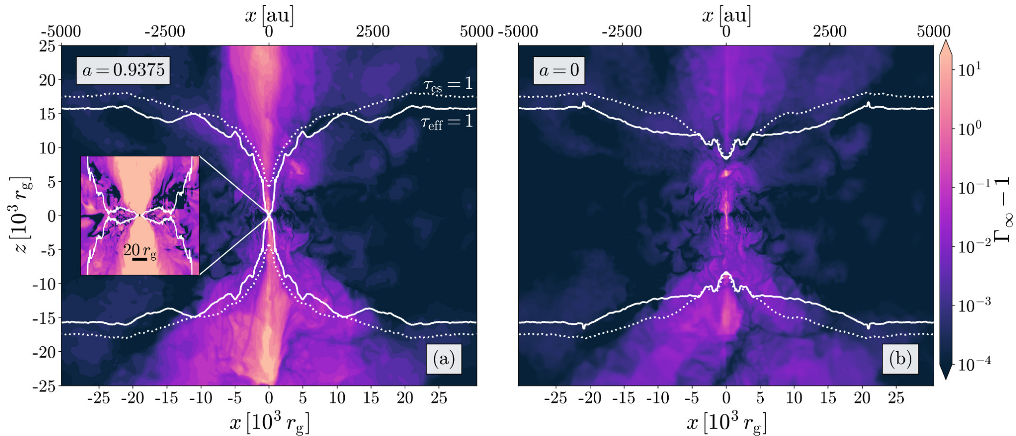
Figure 10. from Nicholas Kaaz et al 2025 Astrophys. J. 979 doi:10.3847/1538-4357/ad9a86 https://dx.doi.org/10.3847/1538-4357/ad9a86 © 2025. The Author(s). Published by the American Astronomical Society.
