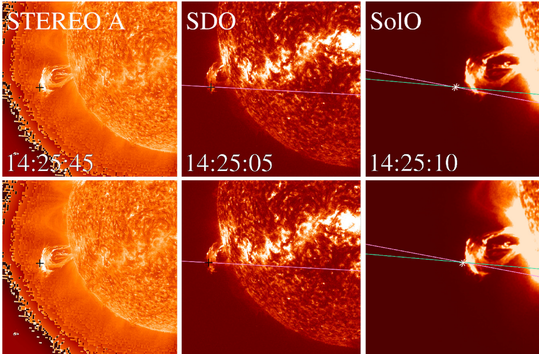
Figure 9. from Abril Sahade et al 2025 Astrophys. J. 978 doi:10.3847/1538-4357/ad96ba https://dx.doi.org/10.3847/1538-4357/ad96ba © 2024. The Author(s). Published by the American Astronomical Society.
