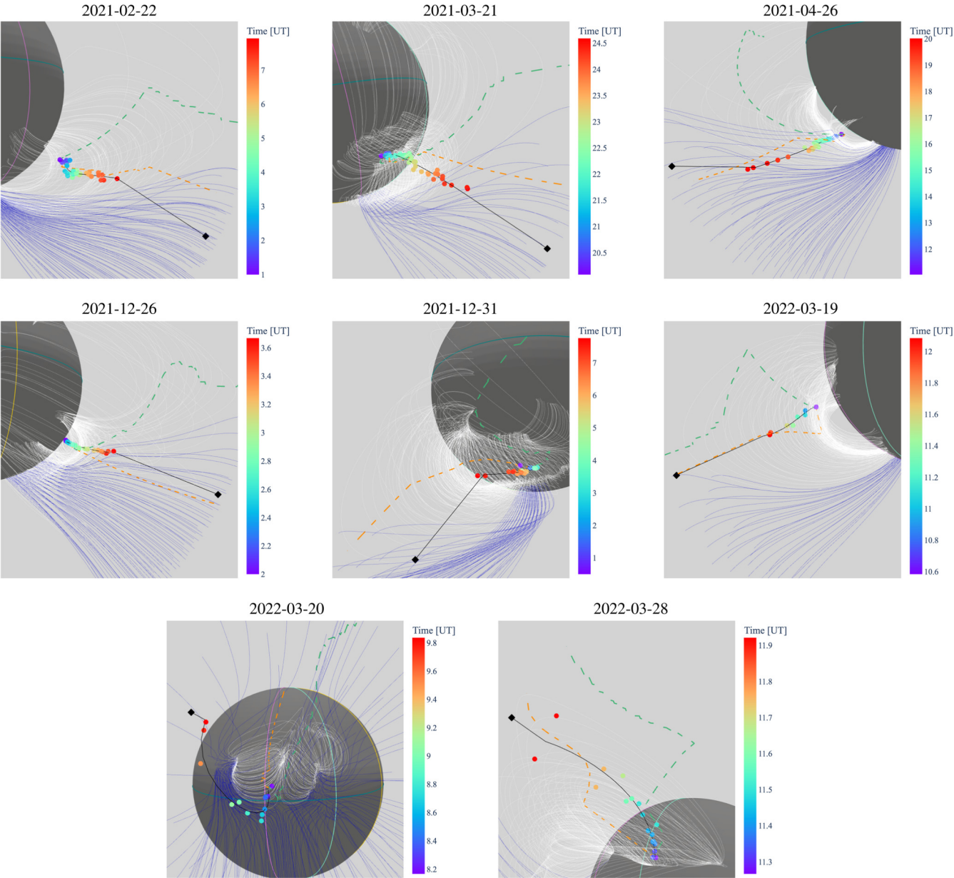
Figure 7. from Abril Sahade et al 2025 Astrophys. J. 978 doi:10.3847/1538-4357/ad96ba https://dx.doi.org/10.3847/1538-4357/ad96ba © 2024. The Author(s). Published by the American Astronomical Society.
