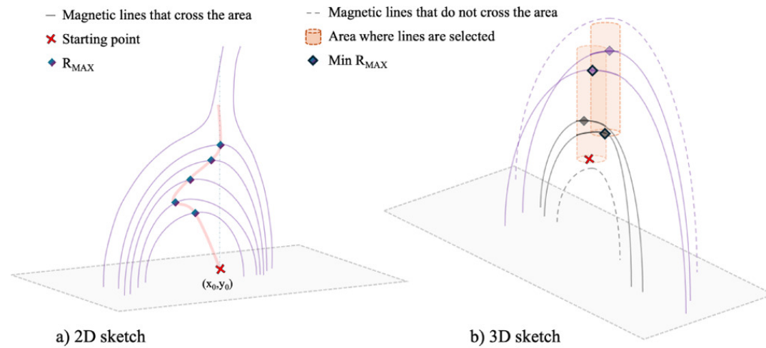
Figure 5. from Abril Sahade et al 2025 Astrophys. J. 978 doi:10.3847/1538-4357/ad96ba https://dx.doi.org/10.3847/1538-4357/ad96ba © 2024. The Author(s). Published by the American Astronomical Society.
