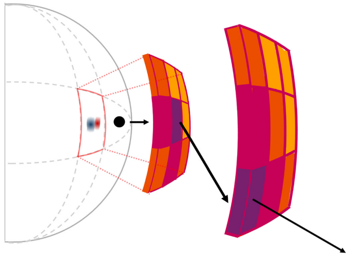
Figure 4. from Abril Sahade et al 2025 Astrophys. J. 978 doi:10.3847/1538-4357/ad96ba https://dx.doi.org/10.3847/1538-4357/ad96ba © 2024. The Author(s). Published by the American Astronomical Society.
