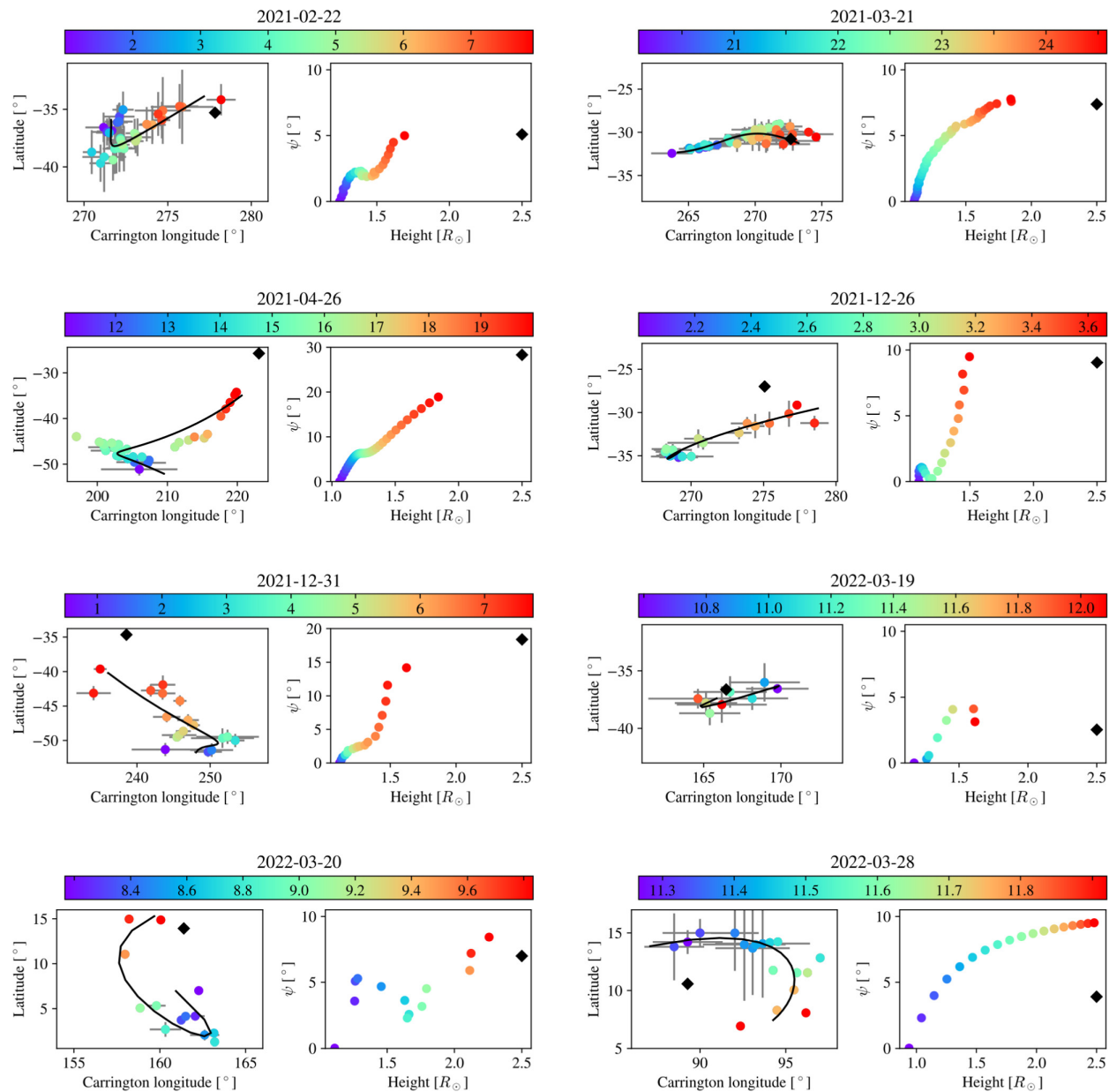
Figure 3. from Abril Sahade et al 2025 Astrophys. J. 978 doi:10.3847/1538-4357/ad96ba https://dx.doi.org/10.3847/1538-4357/ad96ba © 2024. The Author(s). Published by the American Astronomical Society.
