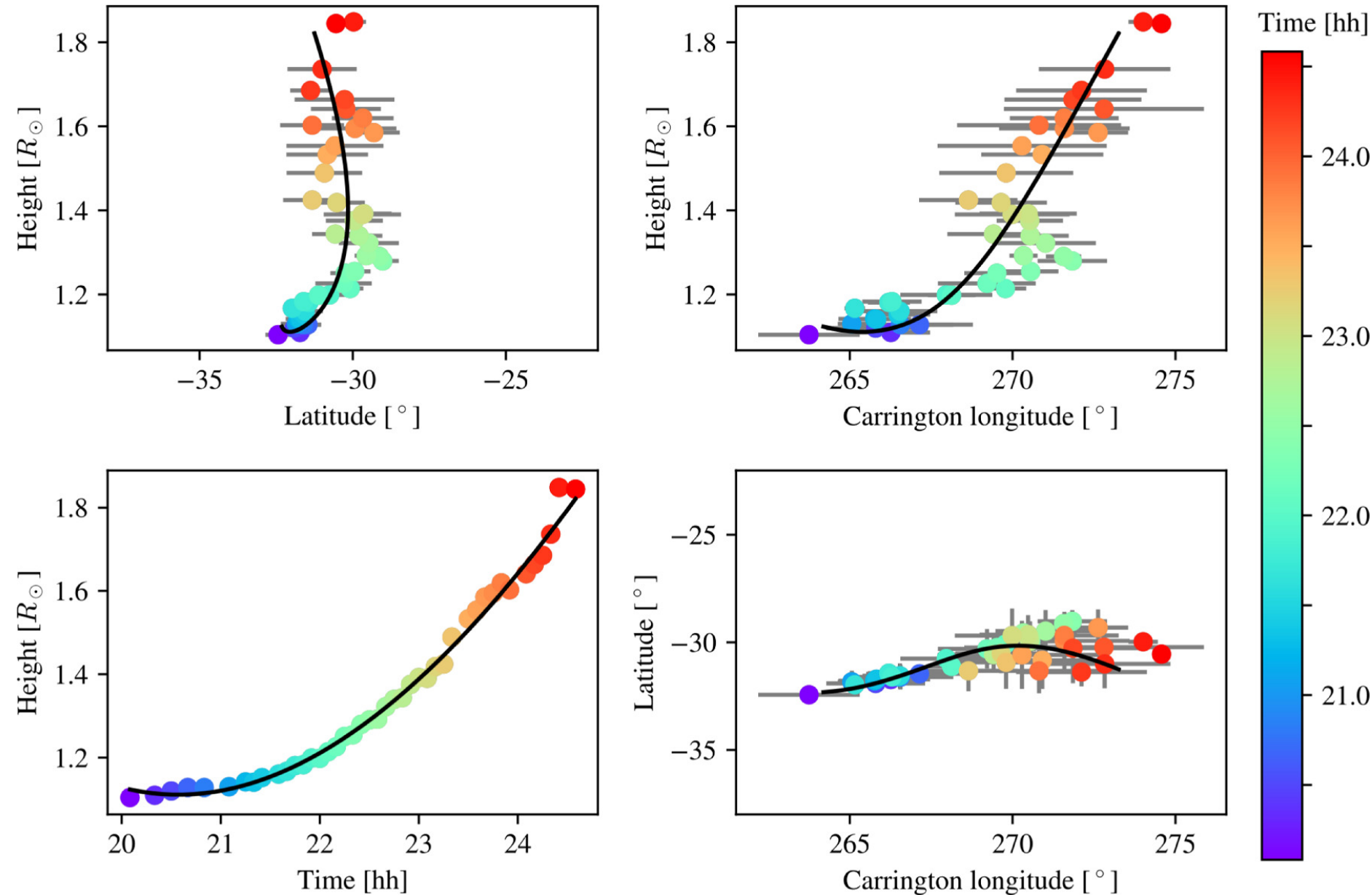
Figure 2. from Abril Sahade et al 2025 Astrophys. J. 978 doi:10.3847/1538-4357/ad96ba https://dx.doi.org/10.3847/1538-4357/ad96ba © 2024. The Author(s). Published by the American Astronomical Society.
