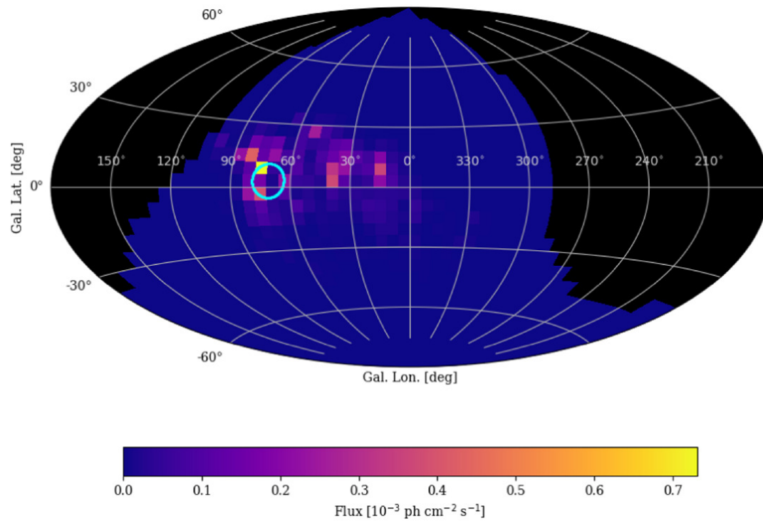
Figure 7. from Jarred M. Roberts et al 2025 Astrophys. J. 979 doi:10.3847/1538-4357/ad968a https://dx.doi.org/10.3847/1538-4357/ad968a © 2025. The Author(s). Published by the American Astronomical Society.
