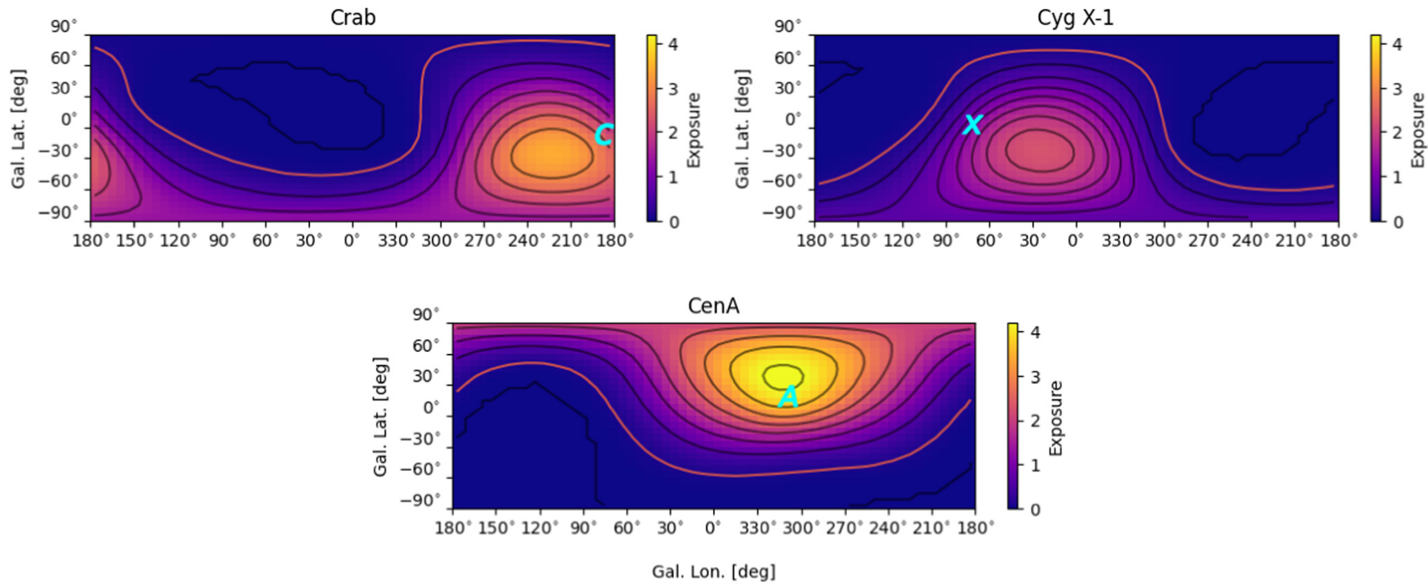
Figure 5. from Jarred M. Roberts et al 2025 Astrophys. J. 979 doi:10.3847/1538-4357/ad968a https://dx.doi.org/10.3847/1538-4357/ad968a © 2025. The Author(s). Published by the American Astronomical Society.
