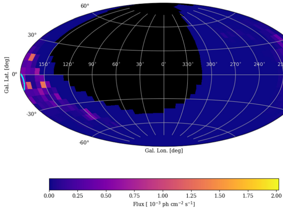
Figure 4. from Jarred M. Roberts et al 2025 Astrophys. J. 979 doi:10.3847/1538-4357/ad968a https://dx.doi.org/10.3847/1538-4357/ad968a © 2025. The Author(s). Published by the American Astronomical Society.
