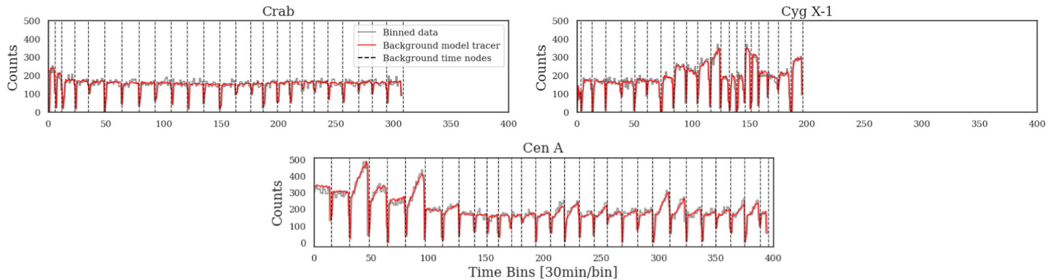
Figure 3. from Jarred M. Roberts et al 2025 Astrophys. J. 979 doi:10.3847/1538-4357/ad968a https://dx.doi.org/10.3847/1538-4357/ad968a © 2025. The Author(s). Published by the American Astronomical Society.
