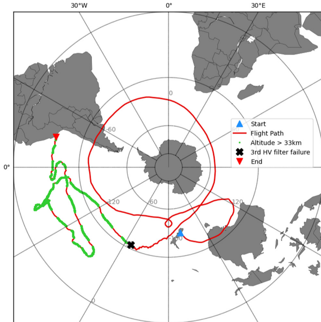
Figure 1. from Jarred M. Roberts et al 2025 Astrophys. J. 979 doi:10.3847/1538-4357/ad968a https://dx.doi.org/10.3847/1538-4357/ad968a © 2025. The Author(s). Published by the American Astronomical Society.
