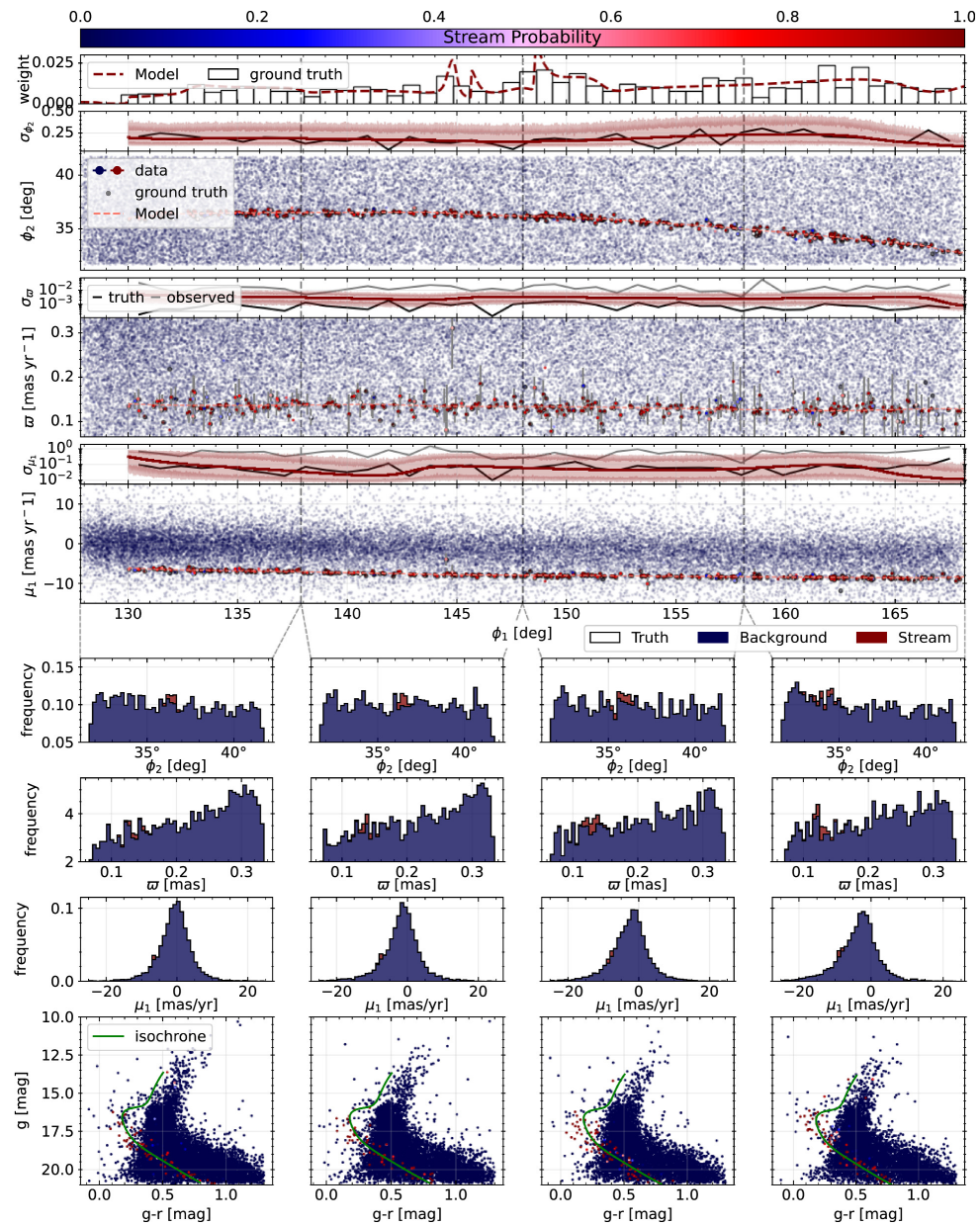
Figure 3. from Nathaniel Starkman et al 2025 Astrophys. J. 980 doi:10.3847/1538-4357/ad94f2 https://dx.doi.org/10.3847/1538-4357/ad94f2 © 2025. The Author(s). Published by the American Astronomical Society.
