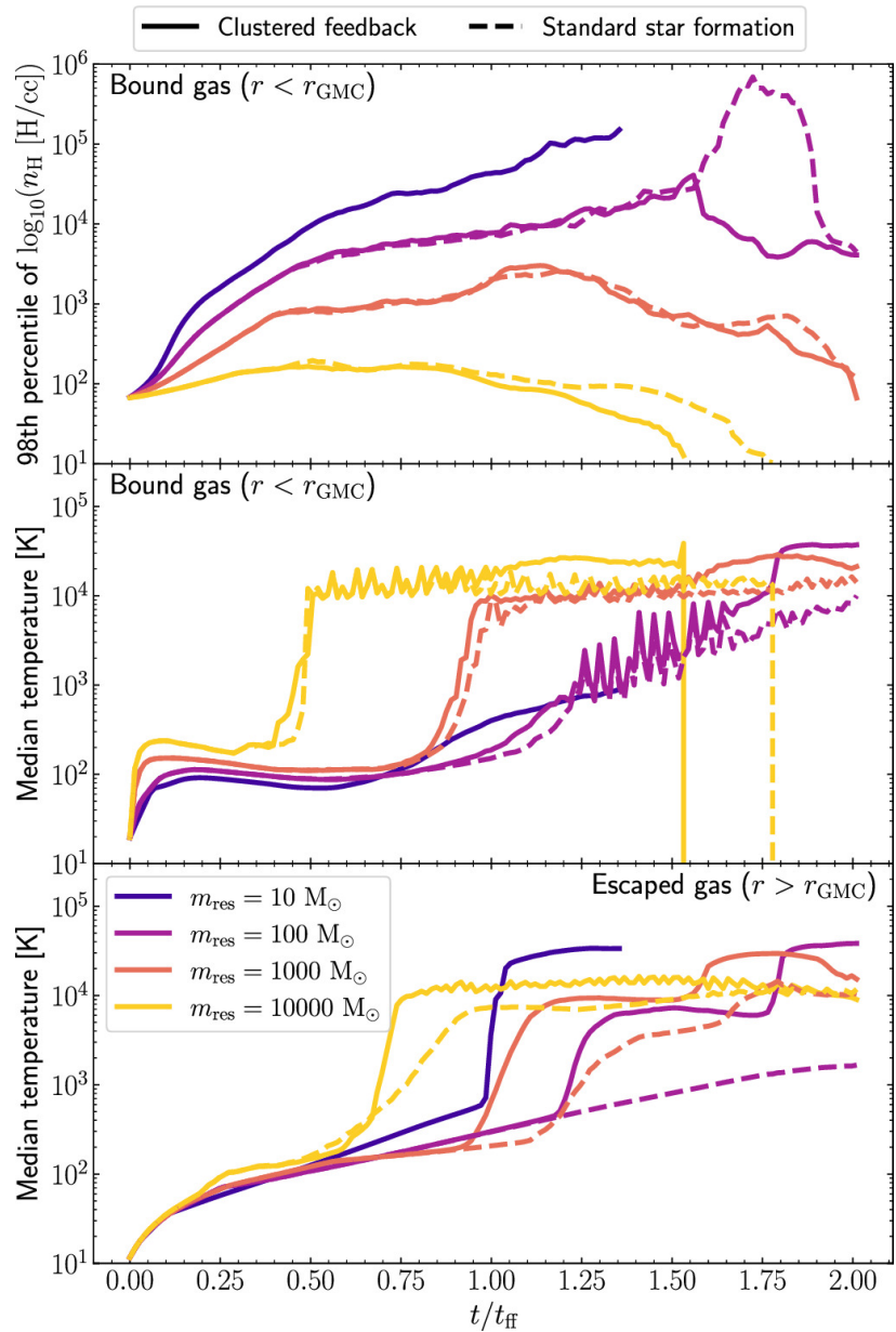
Figure 9. from Marta Reina-Campos et al 2025 Astrophys. J. 978 doi:10.3847/1538-4357/ad909f https://dx.doi.org/10.3847/1538-4357/ad909f © 2024. The Author(s). Published by the American Astronomical Society.
