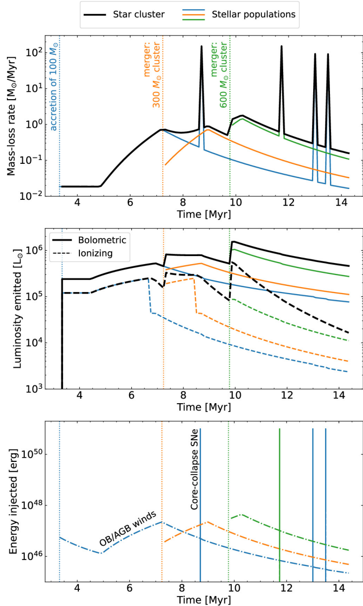
Figure 2. from Marta Reina-Campos et al 2025 Astrophys. J. 978 doi:10.3847/1538-4357/ad909f https://dx.doi.org/10.3847/1538-4357/ad909f © 2024. The Author(s). Published by the American Astronomical Society.
